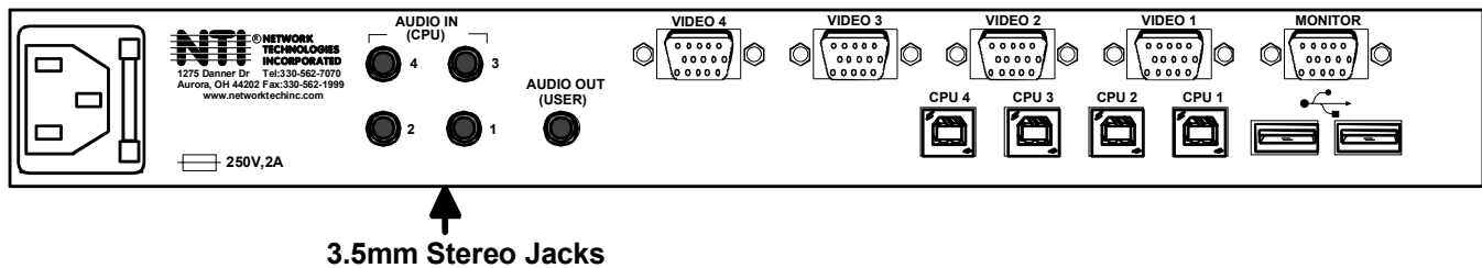
Figure 37- Rear View of UNIMUX-USBV-4O-A
