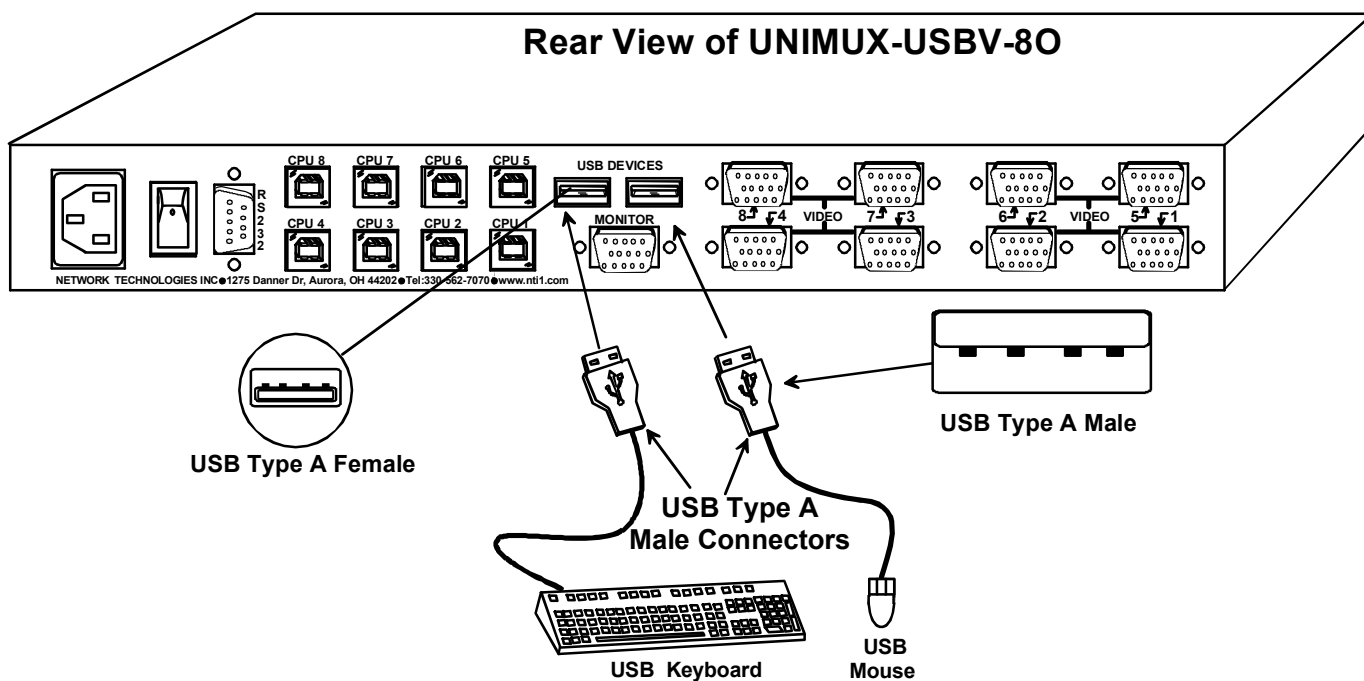
Figure 4- Connect the device(s)
