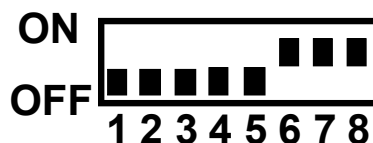
Figure 28- RS232 DIP switches
